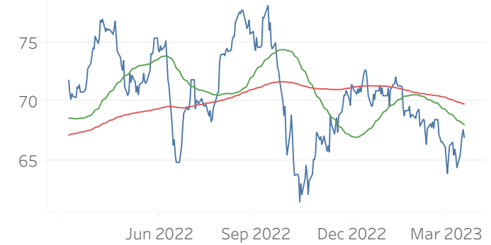
Utilities XLU
