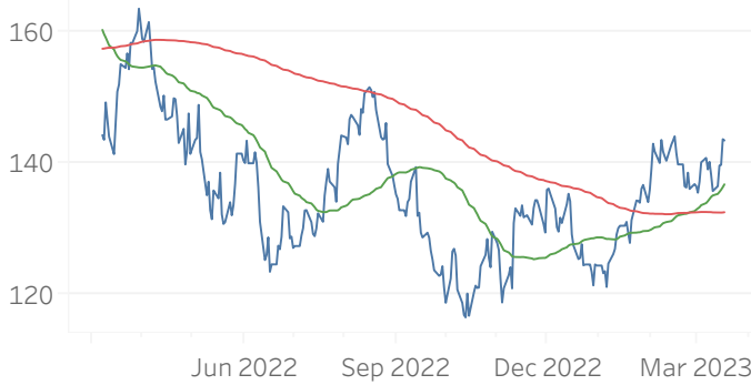
Technology XLK
